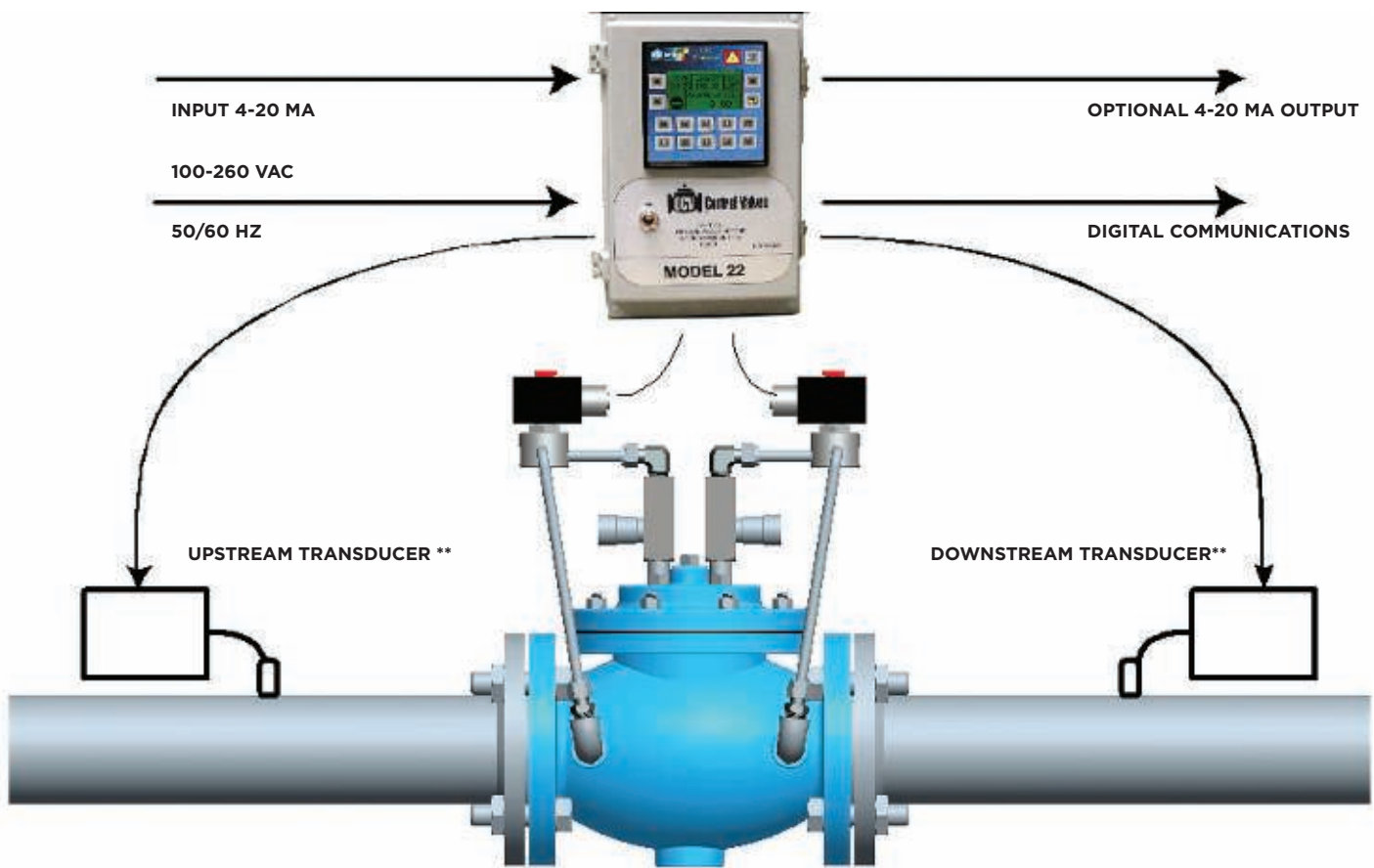
** PRESSURE TRANSDUCER, FLOW METER, LEVEL TRANSMITTER, THERMOCOUPLE OR RTD
