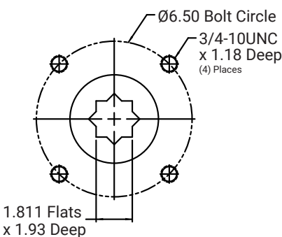
Actuator Mounting Model 240 thru 270
